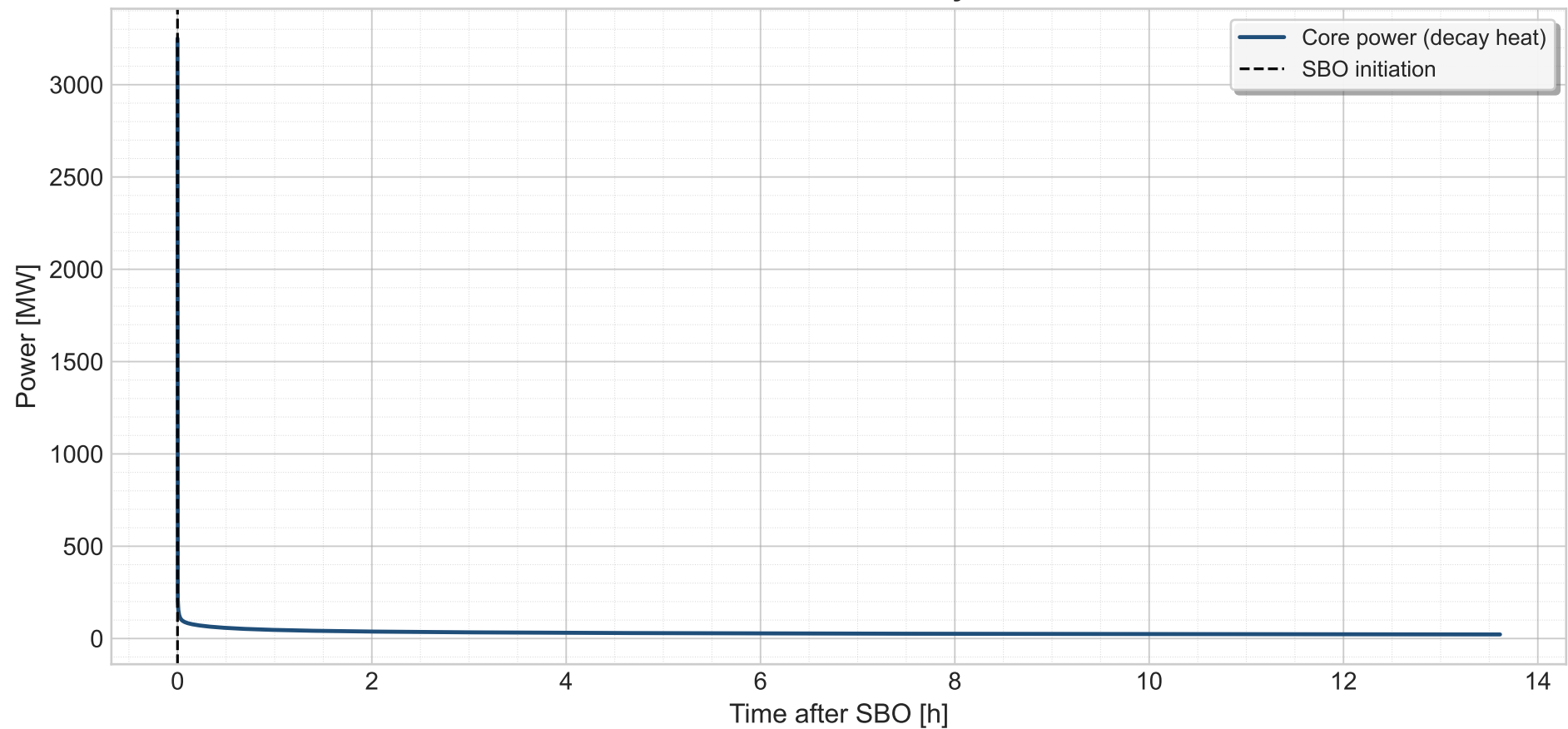
Base Case - Core Decay Heat
